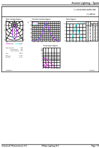
Accent Lighting Spots - CorePro LEDspot 5-65W GU10 840 36D ND
