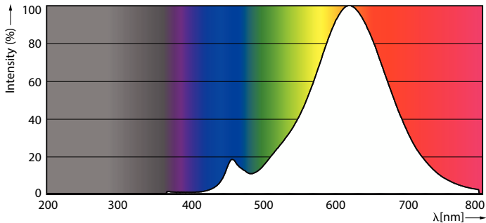
Spectral Power Distribution Colour - CLA LEDBulb ND 7-60W E27 WW ST64 CL
