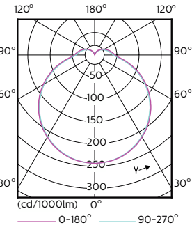
Light Distribution Diagram - 10.5PL-C/T/COR/26V-830/IF13/P/4P/DIM10/1
