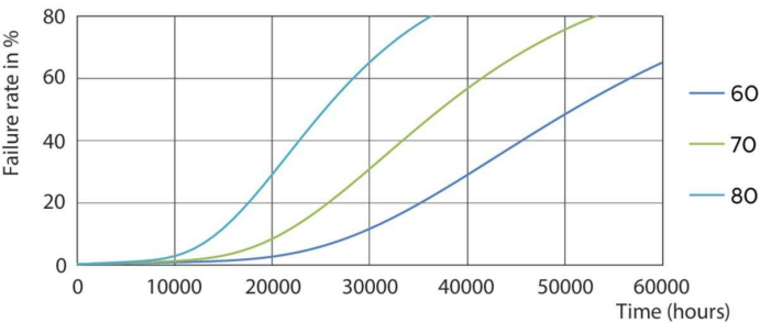
Life Expectancy Diagram - 10.5PL-C/T/COR/26V-830/IF13/P/4P/DIM10/1
