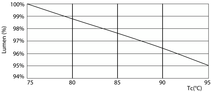
Lumen Maintenance Diagram - 10.5PL-C/T/COR/26V-830/IF13/P/4P/ DIM10/1
