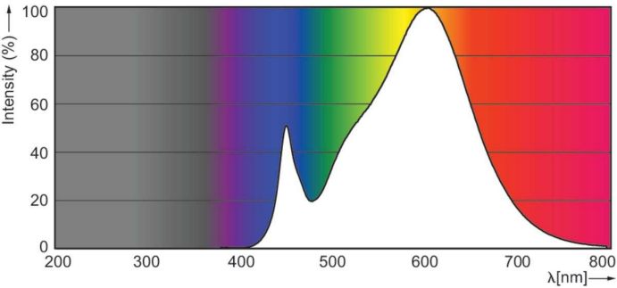
Spectral Power Distribution Colour - 10.5PL-C/T/COR/26V-830/IF13/P/4P/DIM10/1
