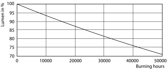
Lumen Maintenance Diagram - 10.5PL-C/T/COR/26V-830/IF13/P/4P/DIM10/1
