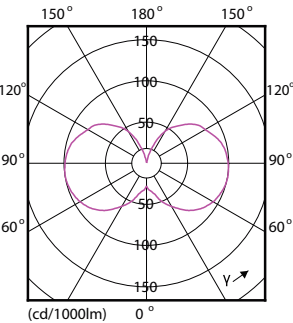
Light Distribution Diagram - CLA LEDBulb SP ND 5-25W E27 GOLD G93 CL
