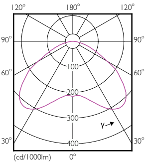
Light Distribution Diagram - TForce Core HB 200-160W E40 865 WB LA
