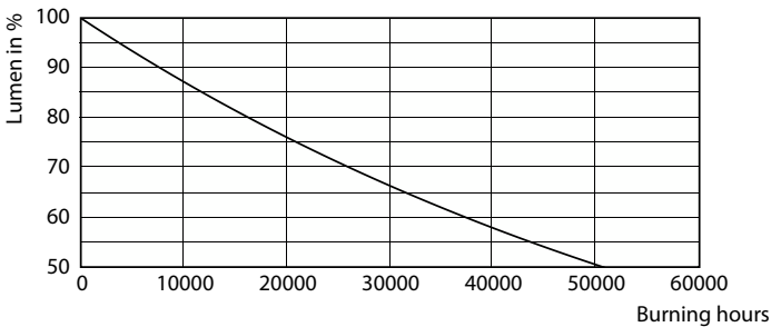
Lumen Maintenance Diagram - TForce Core HB 200-160W E40 865 WB LA
