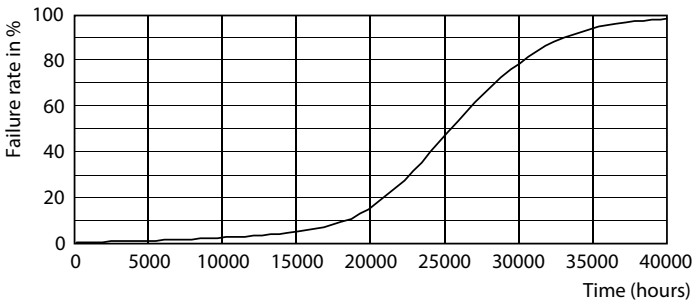
Life Expectancy Diagram - TForce Core HB 200-160W E40 865 WB LA
