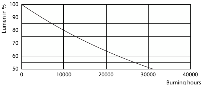
Lumen Maintenance Diagram - LED classic 14W B35 E14 SP GOLD ND 1BC/4
