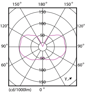
Light Distribution Diagram - LED classic 14W B35 E14 SP GOLD ND 1BC/4
