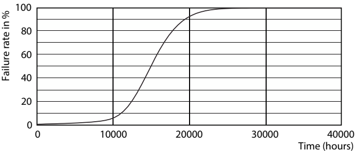
Life Expectancy Diagram - LED classic 14W B35 E14 SP GOLD ND 1BC/4
