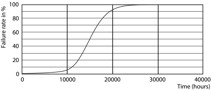
Life Expectancy Diagram - LED classic-giant 25W E27 A160 GOLD ND
