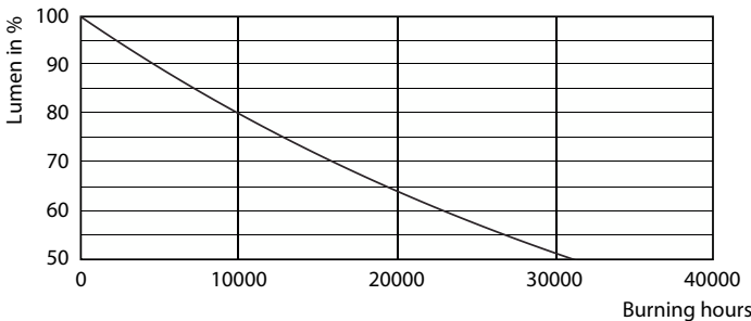
Lumen Maintenance Diagram - LED classic-giant 25W E27 A160 GOLD ND
