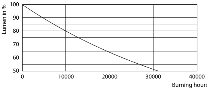
Lumen Maintenance Diagram - LED classic-giant 25W E27 G200 GOLD ND
