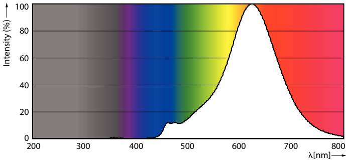
Spectral Power Distribution Colour - LED classic-giant 25W E27 G200 GOLD ND
