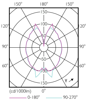
Light Distribution Diagram - LED classic-giant 25W E27 G200 GOLD ND
