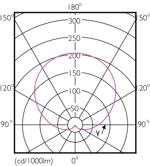
Light Distribution Diagram - LEDBulb 5W E27 6500K W A19 1PF/6 MX
