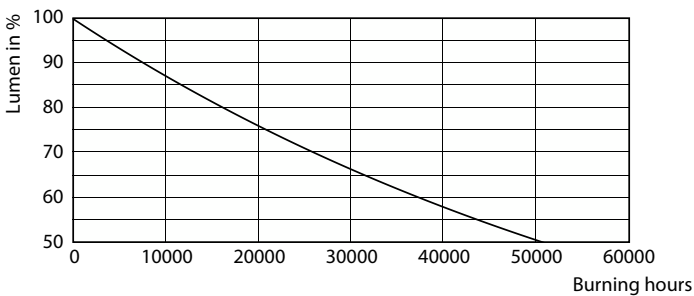
Lumen Maintenance Diagram - LEDBulb 5W E27 6500K W A19 1PF/6 MX
