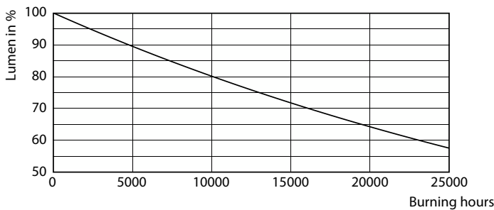
Lumen Maintenance Diagram - CorePro LEDcapsuleLV 0.9-10W G4 830
