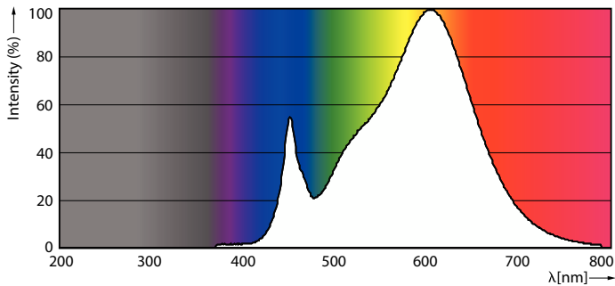
Spectral Power Distribution Colour - CorePro LEDcapsuleLV 0.9-10W G4 830
