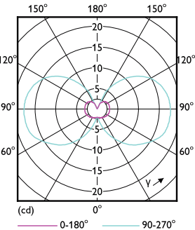
Light Distribution Diagram - CorePro LEDcapsuleLV 0.9-10W G4 830
