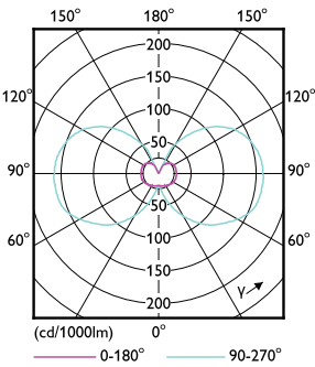
Light Distribution Diagram - CorePro LEDcapsuleLV 1.7-20W G4 827
