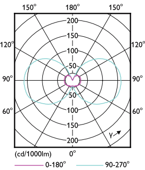
Light Distribution Diagram – CorePro LEDcapsuleLV 1.7-20W G4 830
