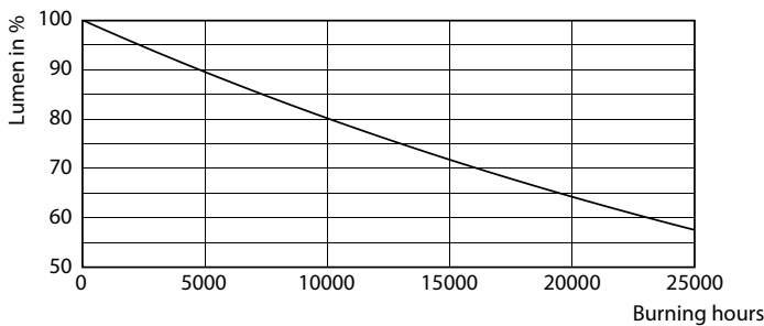
Lumen Maintenance Diagram - CorePro LEDcapsuleLV 1.7-20W G4 830
