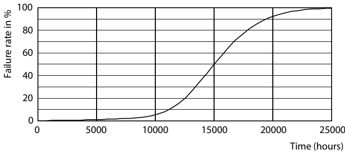
Life Expectancy Diagram - CorePro LEDcapsuleLV 1.7-20W GY6.35 827
