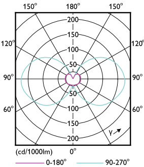
Light Distribution Diagram - CorePro LEDcapsuleLV 1.7-20W GY6.35 827
