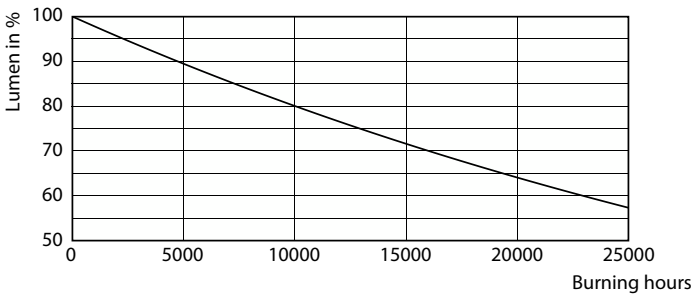
Lumen Maintenance Diagram - CorePro LEDcapsuleLV 1.7-20W GY6.35 827
