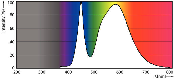
Spectral Power Distribution Colour - LED spot 5-50W 120D 4000K 220V
