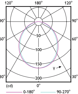
Light Distribution Diagram - LED spot 5-50W 120D 6500K 220V
