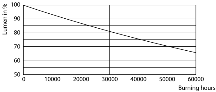
Lumen Maintenance Diagram - 150HB/LED/750/ND NB DL BB 2/1
