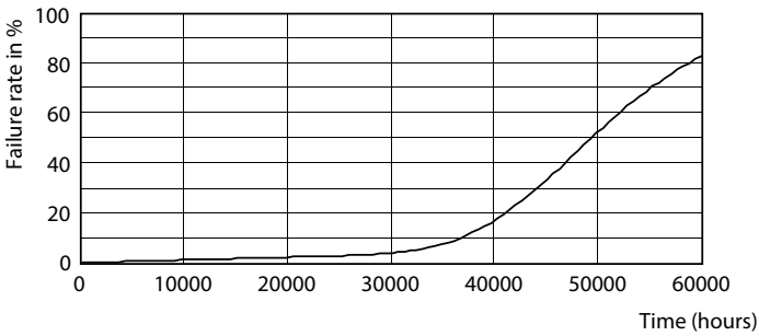
Life Expectancy Diagram - 150HB/LED/750/ND NB DL BB 2/1
