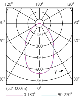
Light Distribution Diagram - 150HB/LED/750/ND NB DL BB 2/1
