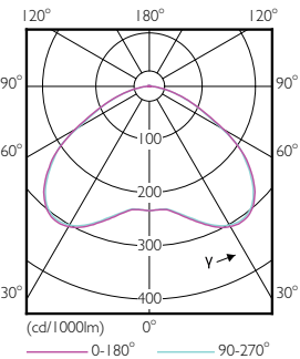
Light Distribution Diagram - 150HB/LED/750/ND WB DL BB 2/1
