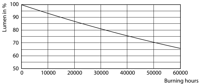
Lumen Maintenance Diagram - 150HB/LED/750/ND WB DL BB 2/1
