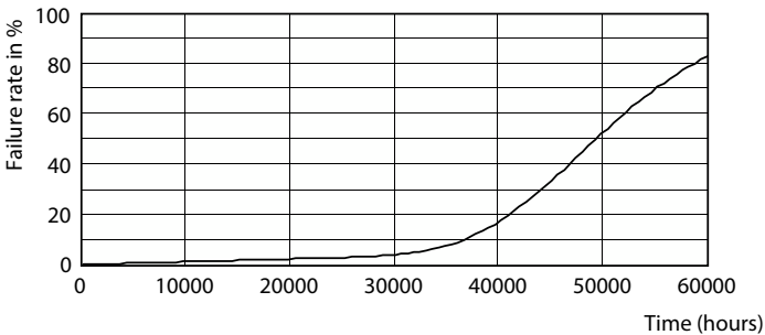
Life Expectancy Diagram - 150HB/LED/750/ND WB DL BB 2/1
