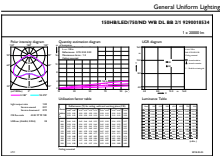
Light Distribution Diagram - 150HB/LED/750/ND WB DL BB 2/1
