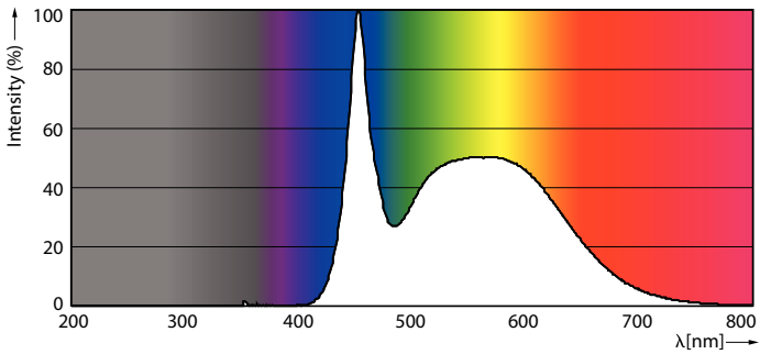
Spectral Power Distribution Colour - ESS LED 7W E27 6500K 230V R63
