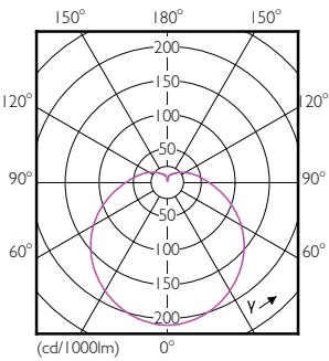
Light Distribution Diagram - ESS LED 7W E27 6500K 230V R63
