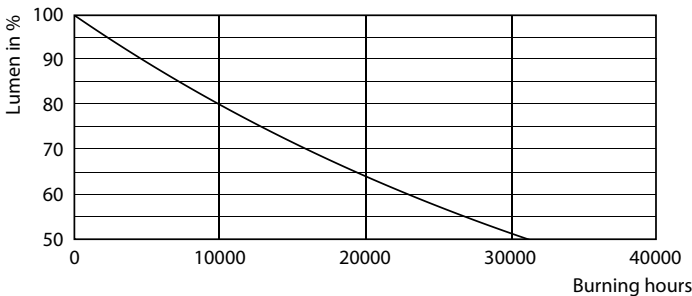
Lumen Maintenance Diagram - ESS LED 7W E27 6500K 230V R63
