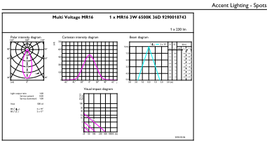
Light Distribution Diagram - ESS LED MR16 3-35W 36D 865 SO 100-240V
