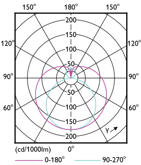
Light Distribution Diagram - 12T8/PER/48-850/BB18/G 10/1 FB
