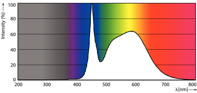
Spectral Power Distribution Colour - 12T8/PER/48-850/BB18/G 10/1 FB
