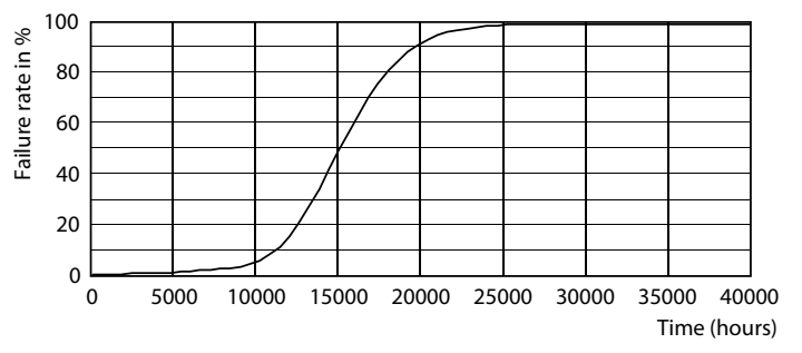
Life Expectancy Diagram - LED PLC 7.5W 840 2P G24d
