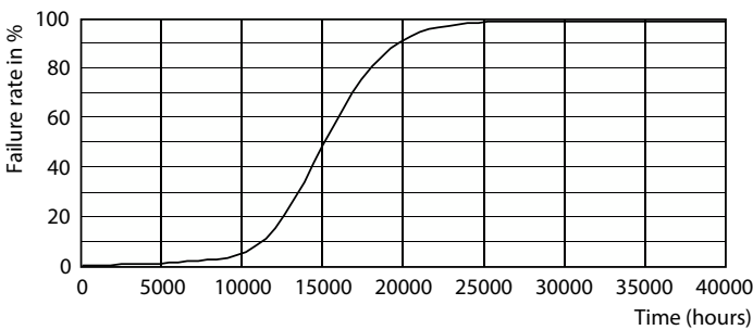
Life Expectancy Diagram - LED PLC 7.5W 865 2P G24d
