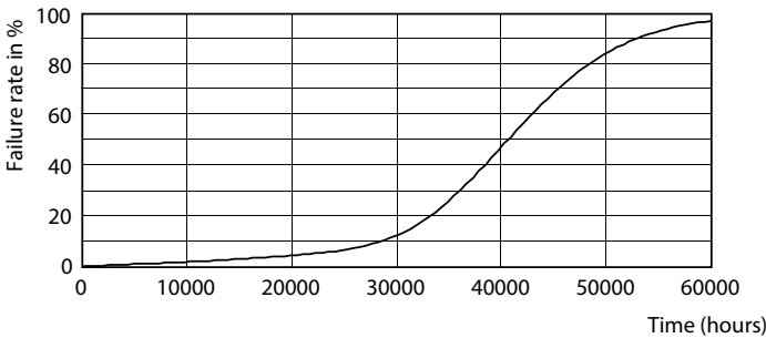
Life Expectancy Diagram - MASTER LED 7-50W 940 MR16 24D Dim
