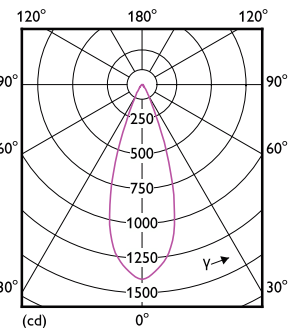
Light Distribution Diagram - MASTER LED 7-50W 940 MR16 36D Dim
