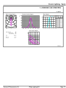
Accent Lighting Spots - MAS LEDspotLV D 8-50W 827 MR16 24D
