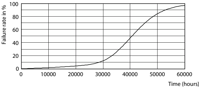
Life Expectancy Diagram - MAS LEDspotLV D 8-50W 840 MR16 24D
