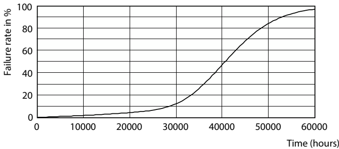
Life Expectancy Diagram - MAS LEDspotLV D 8-50W 827 MR16 36D
