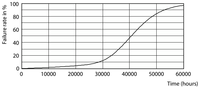
Life Expectancy Diagram - MAS LEDspotLV D 8-50W 830 MR16 36D
