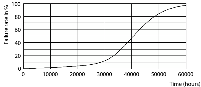
Life Expectancy Diagram - MASTER LED 8-50W+ 840 MR16 36D Dim
