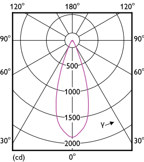
Light Distribution Diagram - MASTER LED 8-50W+ 840 MR16 36D Dim
