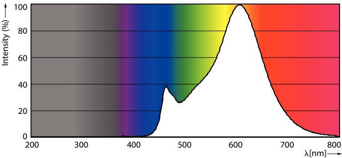
Spectral Power Distribution Colour - CLA LEDBulb D 12-100W A67 E27 827 CL
