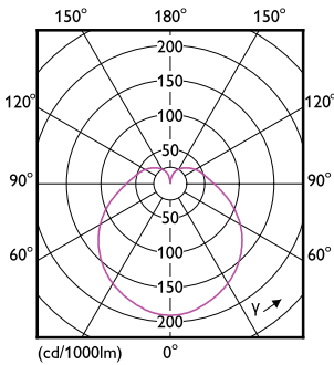
Light Distribution Diagram - 5PL-C/LED/13V/827/IF5/P/2P 20/1
