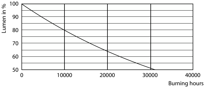
Lumen Maintenance Diagram - CorePro LED bulb ND 19.5-150W A67E27 827
