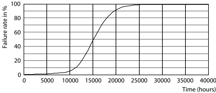
Life Expectancy Diagram - CorePro LED bulb ND 19.5-150W A67E27 827
