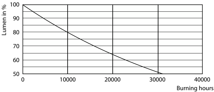
Lumen Maintenance Diagram - CorePro LED bulb ND 17.5-150W A67E27 865
