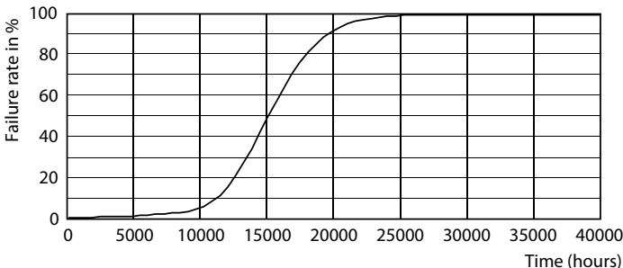
Life Expectancy Diagram - CorePro LED bulb ND 17.5-150W A67E27 865
