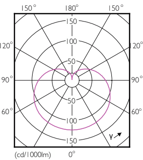
Light Distribution Diagram - CorePro LED bulb ND 17.5-150W A67E27 865
