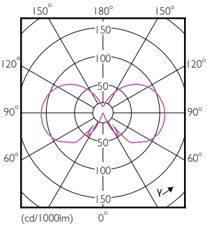
Light Distribution Diagram - CLA LEDBulb D 8-60W G93 E27 827 CL
