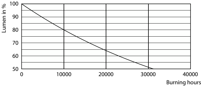
Lumen Maintenance Diagram - CLA LEDBulb D 8-60W G93 E27 827 CL
