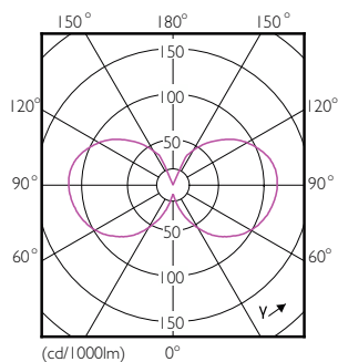
Light Distribution Diagram - CLA LEDBulb D 8-50W G120 E27 822 GOLD
