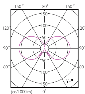
Light Distribution Diagram - CLA LEDLuster D 5-32W P45 E14 822 GOLD
