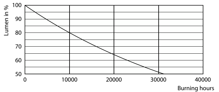
Lumen Maintenance Diagram - CLA LEDLuster D 5-32W P45 E14 822 GOLD
