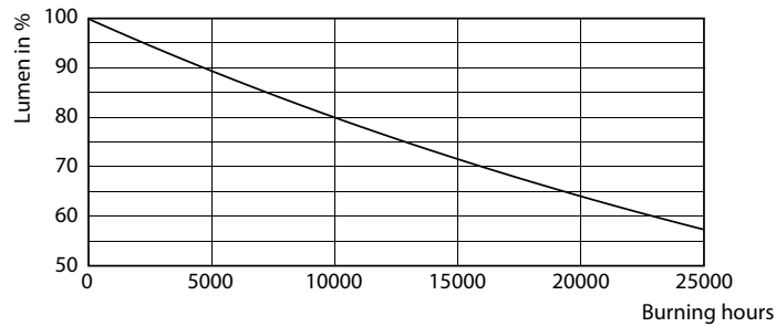
Lumen Maintenance Diagram - CorePro LEDcapsuleLV 2.5-28W G4 827
