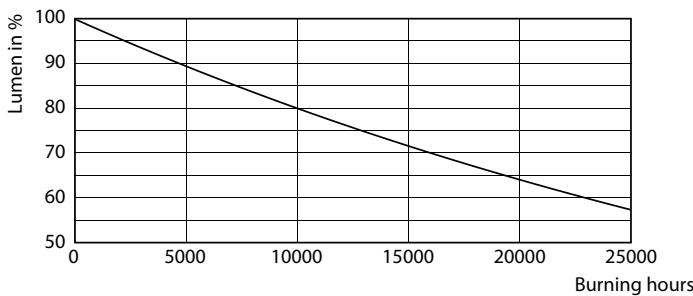
Lumen Maintenance Diagram - CorePro LEDcapsuleLV 2.5-28W G4 827
