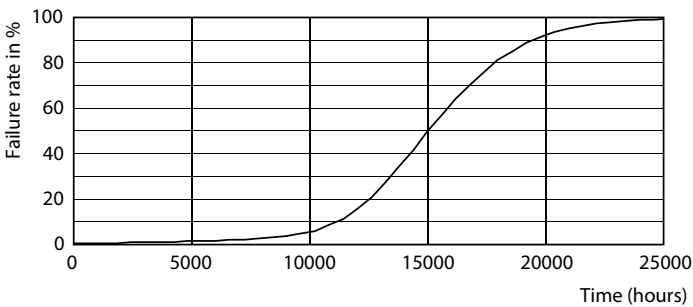
Life Expectancy Diagram - CorePro LEDcapsuleLV 2.5-28W G4 827
