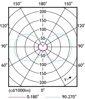
Light Distribution Diagram - CorePro LEDcapsuleLV 2.5-28W G4 827
