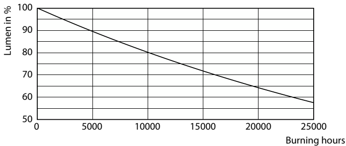
Lumen Maintenance Diagram - CorePro LEDcapsule ND 3.2-40W G9 827
