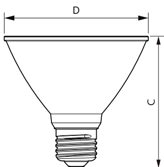
Plastic PAR30s 1100lm 25D 2700K E27 ND
