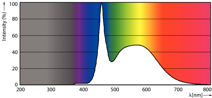
Spectral Power Distribution Colour - Master LED 12-120W PAR30s 865 25D EER1
