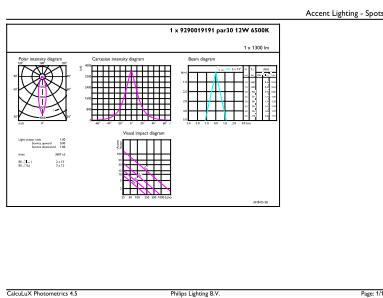
12-120W E26 PAR30S 25D 865 6500K
