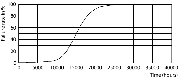
Life Expectancy Diagram - Master LED 12-120W PAR30s 865 25D EER1
