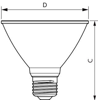
Plastic PAR30s 1100lm 25D 6500K E27 ND
