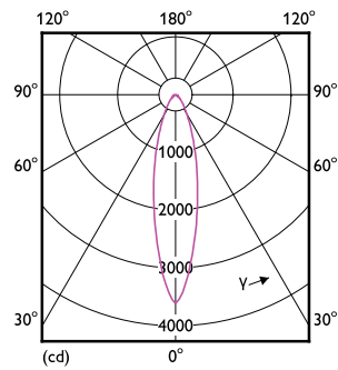
12-120W E26 PAR30S 25D 827 2700K
