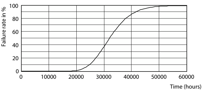
Life Expectancy Diagram - CorePro LED PLL HF 24W 865 4P 2G11
