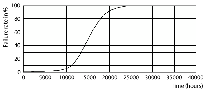
Life Expectancy Diagram - CLA LEDBulb D 8-50W A60 E27 822 GOLD
