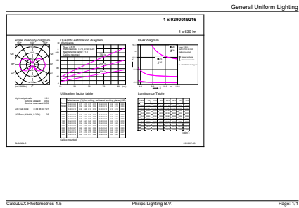
General uniform lighting - CLA LEDBulb D 8-50W A60 E27 822 GOLD
