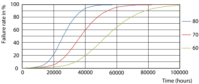
Life Expectancy Diagram - MAS LEDtube 1500mm UO 24W 830 T8 G I
