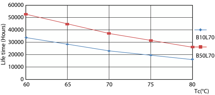
Life Expectancy Diagram - MAS LEDtube 1500mm UO 24W 830 T8 G I
