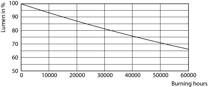
Lumen Maintenance Diagram - MAS LEDtube 1500mm UO 24W 830 T8 G I
