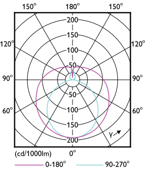
Light Distribution Diagram - MAS LEDtube 1500mm UO 24W 830 T8 G I
