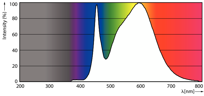
Spectral Power Distribution Colour - TForce LED HB MV ND 120-100W E40 840 WB
