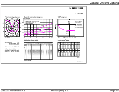
General uniform lighting – 7.5G63/modern/840/CL/G/DIM 2/1CT
