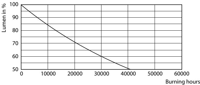
Lumen Maintenance Diagram - TForce Core HB MV ND 26-24W E27 830
