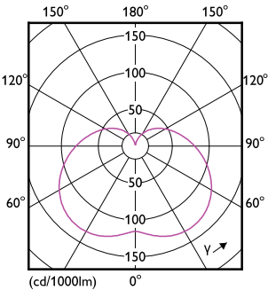
Light Distribution Diagram - TForce Core HB MV ND 26-24W E27 830
