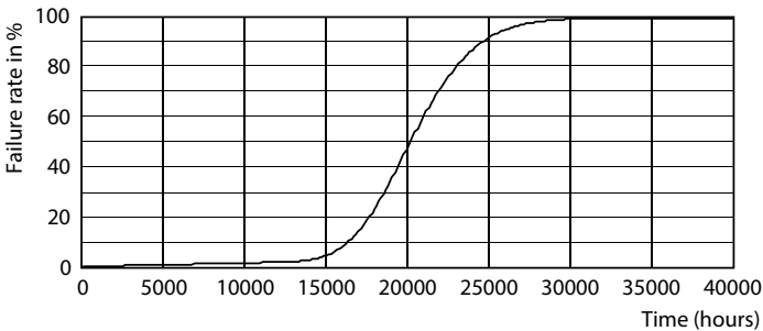
Life Expectancy Diagram - TForce Core HB MV ND 26-24W E27 830
