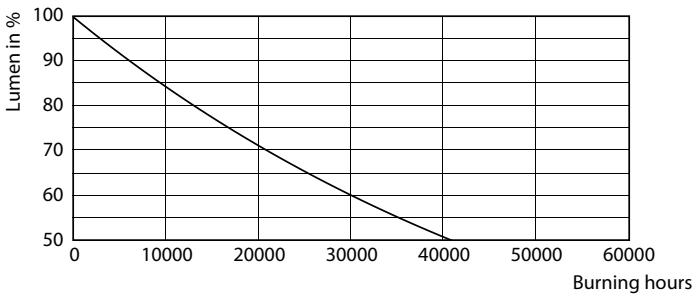
Lumen Maintenance Diagram - TForce Core HB MV ND 48-42W E27 830
