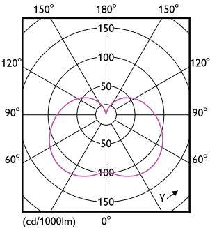
Light Distribution Diagram - TForce Core HB MV ND 48-42W E27 830
