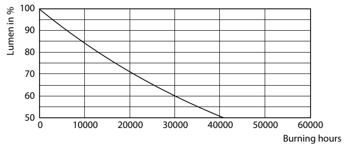
Lumen Maintenance Diagram - TForce Core HB 50-50W E27 840 RCA
