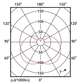
Light Distribution Diagram - TForce Core HB 50-50W E27 840 RCA
