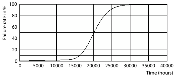
Life Expectancy Diagram - TForce Core HB 50-50W E27 840 RCA
