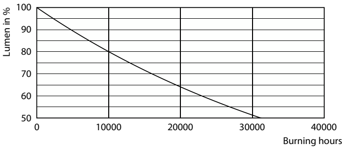
Lumen Maintenance Diagram - Essential LED 12-100W PAR30s 865 25D KR
