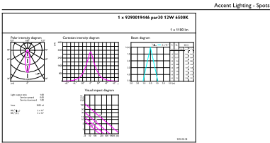
Light Distribution Diagram - Essential LED 12-100W PAR30s 865 25D KR
