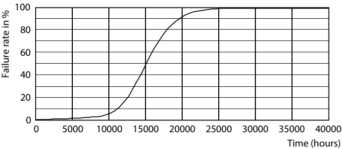
Life Expectancy Diagram - Essential LED 12-100W PAR30s 865 25D KR
